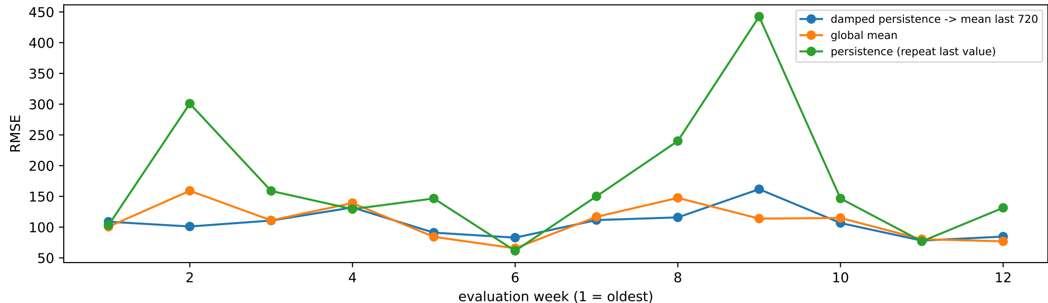
RMSE of each evaluation week — the week matters more than the method
